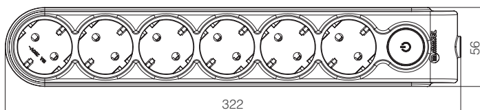
6 Gang Earthed Socket with Switch
