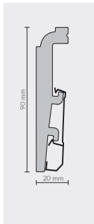
P0911 90x20 mm SKIRTING 5905167734612 2,4 m 24 m 504 m
