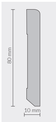
SO810 / WHITE 80x10mm SKIRTING 5905167817759
