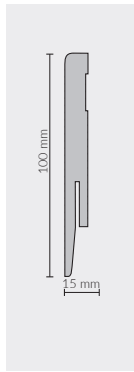
GP1001 100x15 mm SKIRTING 5905167766682 🚚2,42 m 📦24,2 m 🏠1016,4 m
