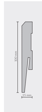
MP1001 100x15 mm SKIRTING 5905167674376 📏 2,42 m 📦 24,2 m 📦 847 m
