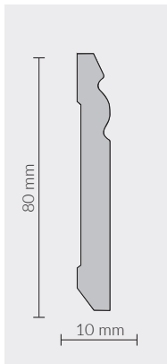
SO820 / WHITE 80x10mm SKIRTING 5905167817780
