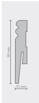
MP0802 80x15 mm SKIRTING 5905167674352 📏 2,42 m 📦 24,2 m 📦 847 m
