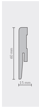
MP0602 60x15 mm SKIRTING 5905167754986 📏 2,42 m 📦 24,2 m 📦 1161,6m
