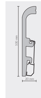
P1020 100x20 mm SKIRTING 5905167734643 2,4 m 24 m 504 m
