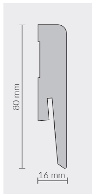
ML 0801 / WHITE 80x16mm SKIRTING 5905167817810
