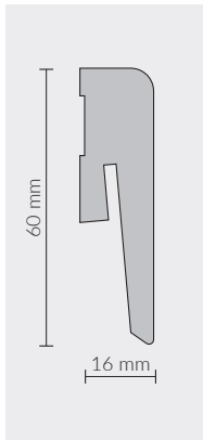
ML0602 / WHITE 60x16mm SKIRTING 5905167817803
