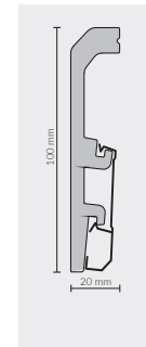
P1010 100x20 mm SKIRTING 5905167734629 2,4 m 24 m 504 m
