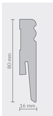
ML0802/ WHITE 80x16mm SKIRTING 5905167817858
