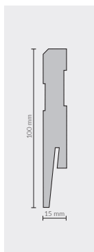
MP1002 100x15 mm SKIRTING 5905167674383 📏 2,42 m 📦 24,2 m 📦 847 m
