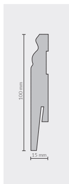
MP1003 100x15 mm SKIRTING 5905167674390 📏 2,42 m 📦 24,2 m 📦 847 m
