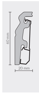
P0620 60x20 mm SKIRTING 5905167755662 2,4 m 21,8 m 672 m
