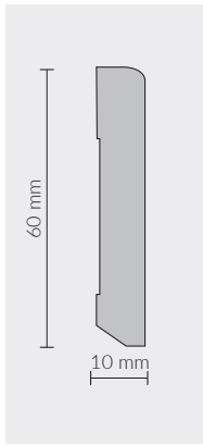
SO611 / WHITE 60x10 SKIRTING 5905167817742
