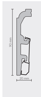
P0910 90x20 mm SKIRTING 5905167734605 2,4 m 24 m 504 m
