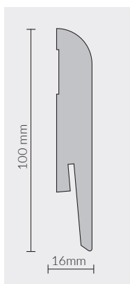
ML1004/ WHITE 100x16mm SKIRTING 5905167817865
