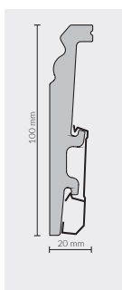
P1030 100x20 mm SKIRTING 5905167755686 2,4 m 24 m 504 m
